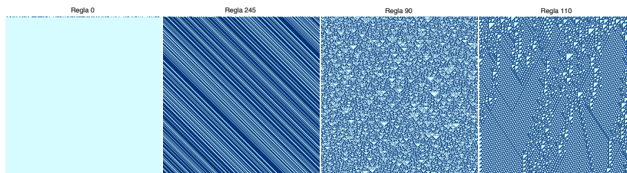
Figure 1: Wolfram classes
